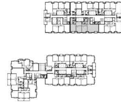
FIRST-KEY-PLAN
