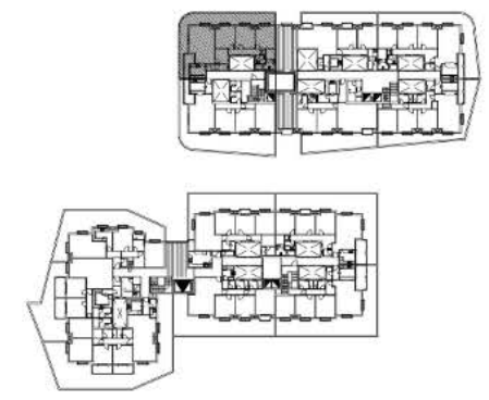
GROUND-KEY-PLAN
