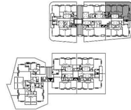
GROUND-KEY-PLAN
