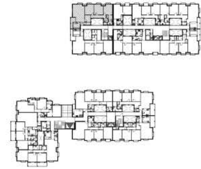
FIRST-KEY-PLAN
